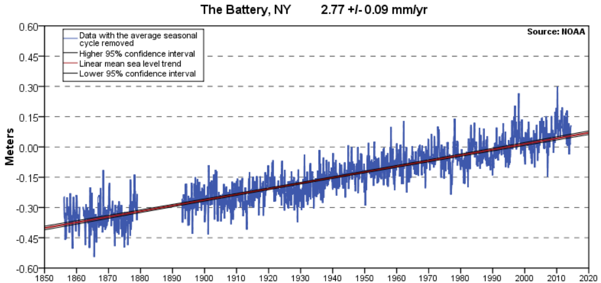
Fig. 1. The trend in sea level at the Battery, New York City. Graphic Credit: NOAA ( http://tidesandcurrents.noaa.gov/sltrends/sltrends_station.shtml?stnid=8518750 )
